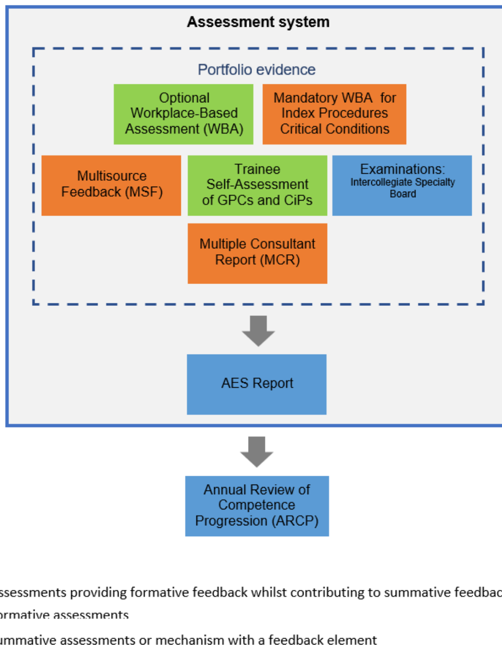
Figure 3: Assessment framework
